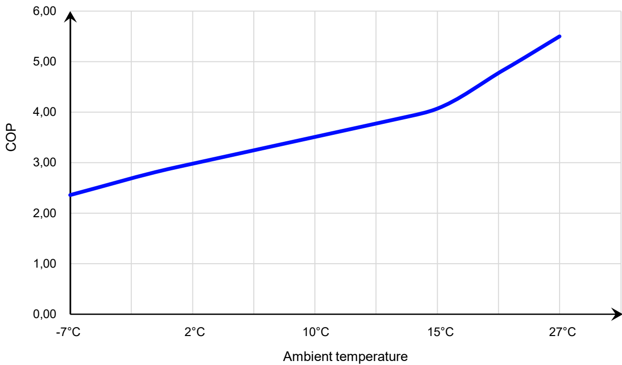
34-180622 COP Curve
